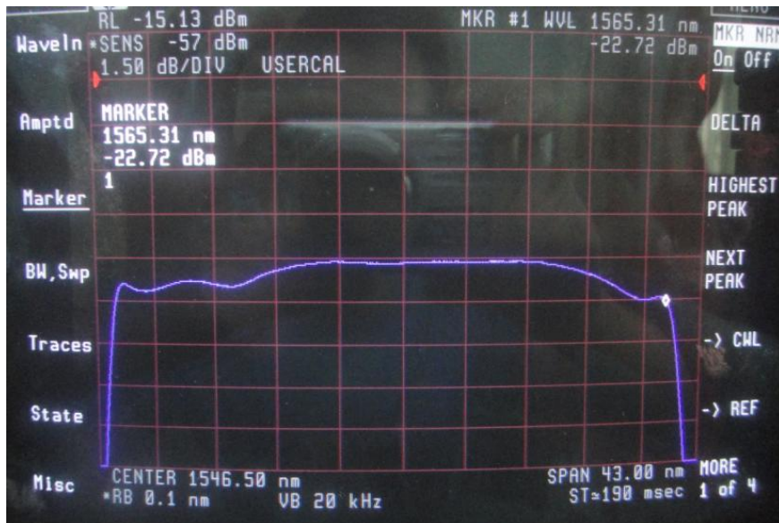
13dBm output spectrum with GFF \leq 1.5 dB
