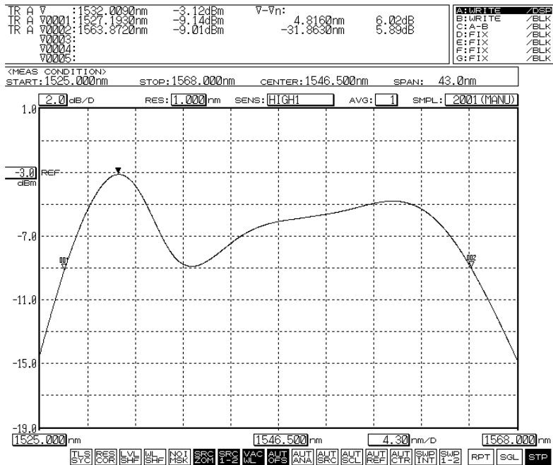
15dBm output spectrum without GFF
